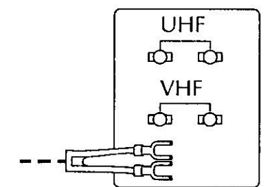
Twin-Lead Antenna
